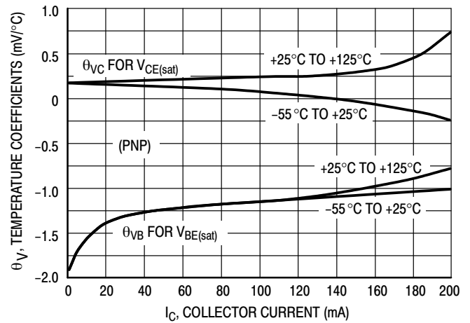
Figure 32. Temperature Coefficients
